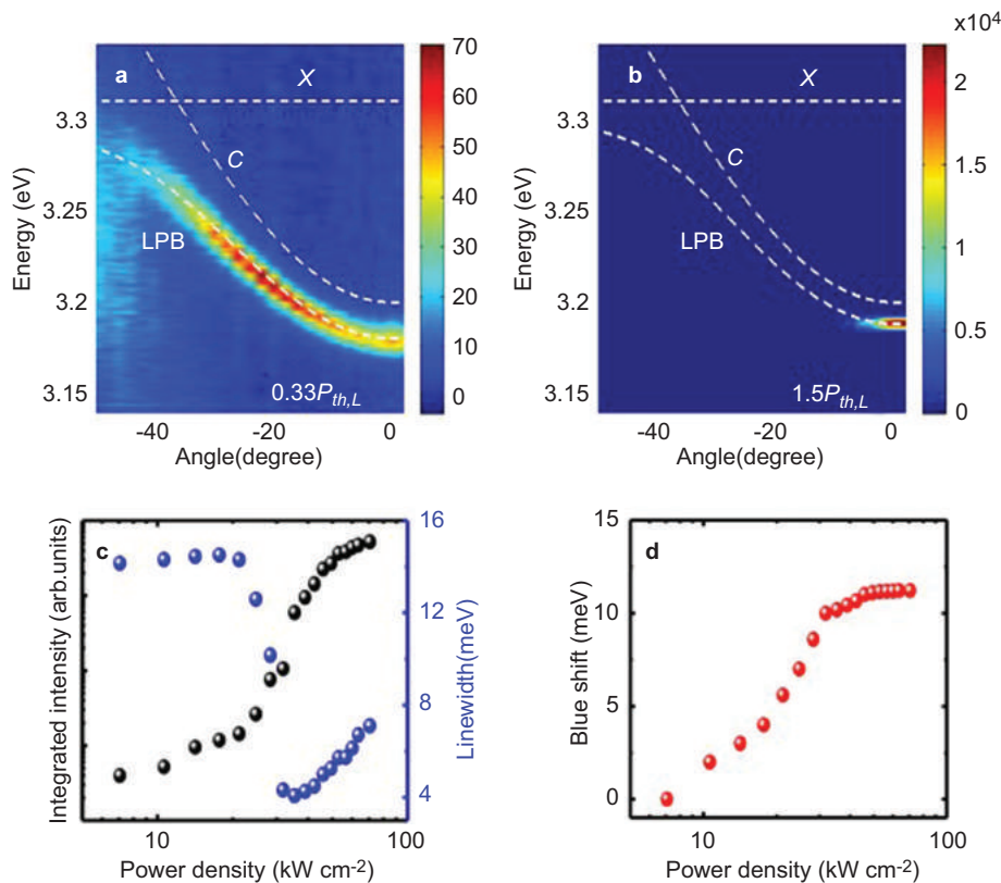
Figure 4 The color maps of the angular dispersions from the measured PL spectra at (a) 0.33P_{th,L} and (b) 1.5P_{th,L} for the case of \delta = -109 \text{ meV} at RT. (c) The integrated emission intensity and emission linewidth and (d) the energy blueshift of the polariton versus the pumping density for the large detuning case ( \delta = -109 \text{ meV} ) at RT. PL, photoluminescence; RT, room temperature.
